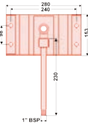
*All Dimensions are in (mm)
